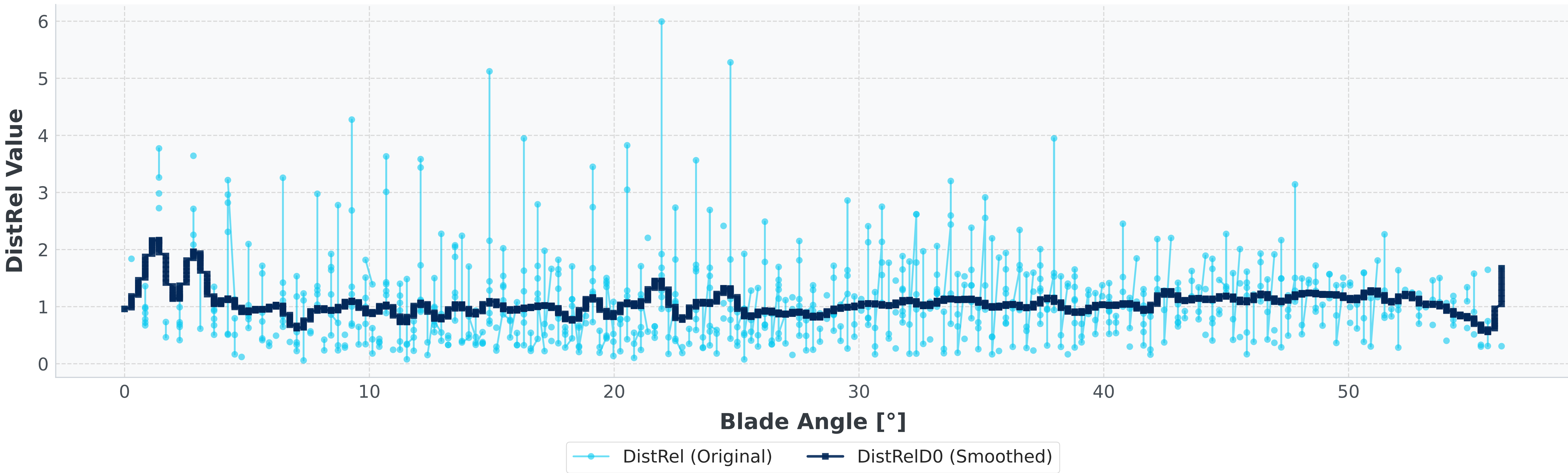
Cavity - DistRel (BLD Phase Averaged)
